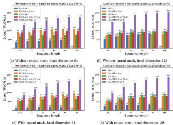
Figure F.11.3: Official benchmark of FlashAttention and FlashAttention-2 on an NVIDIA A100 GPU card, reproduced from https://github.com/Dao-AILab/flash-attention .
