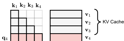
Figure F11.4: To compute masked self-attention on a new token, most of the previous computation can be reused (in gray). This is called the KV cache .
