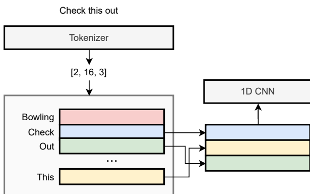
Figure F.8.4: A lookup table to convert a sequence of tokens' IDs to their corresponding embeddings: the input is a list, the output is a matrix. The embeddings (shown inside the box) can be trained together with all the other parameters via gradient descent. We assume the size of the vocabulary is n = 16 .
