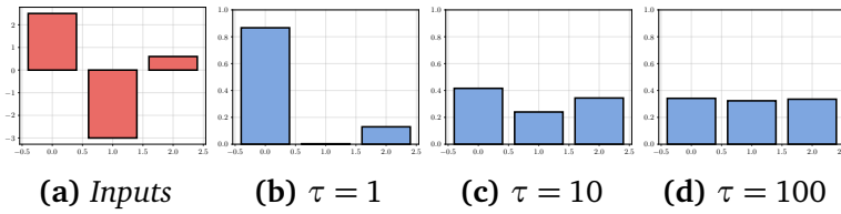
Figure F.4.3: Example of softmax applied to a three-dimensional vector (a), with temperature set to 1 (b), 10 (c), and 100 (d). As the temperature increases, the output converges to a uniform distribution. Note that inputs can be both positive or negative, but the outputs of the softmax are always constrained in [0, 1] .
